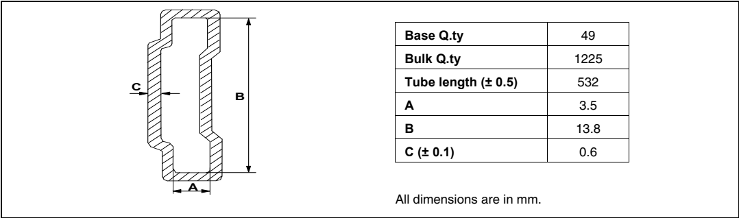
Figure 36. PowerSSO-24 tube shipment (no suffix)
