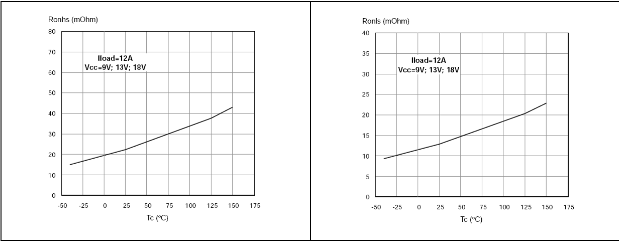
Figure 25. On state high side resistance vs T_{case} Figure 26. On state low side resistance vs T_{case}
