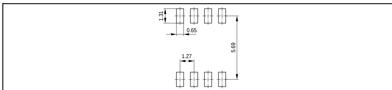
Figure 17 Footprint
