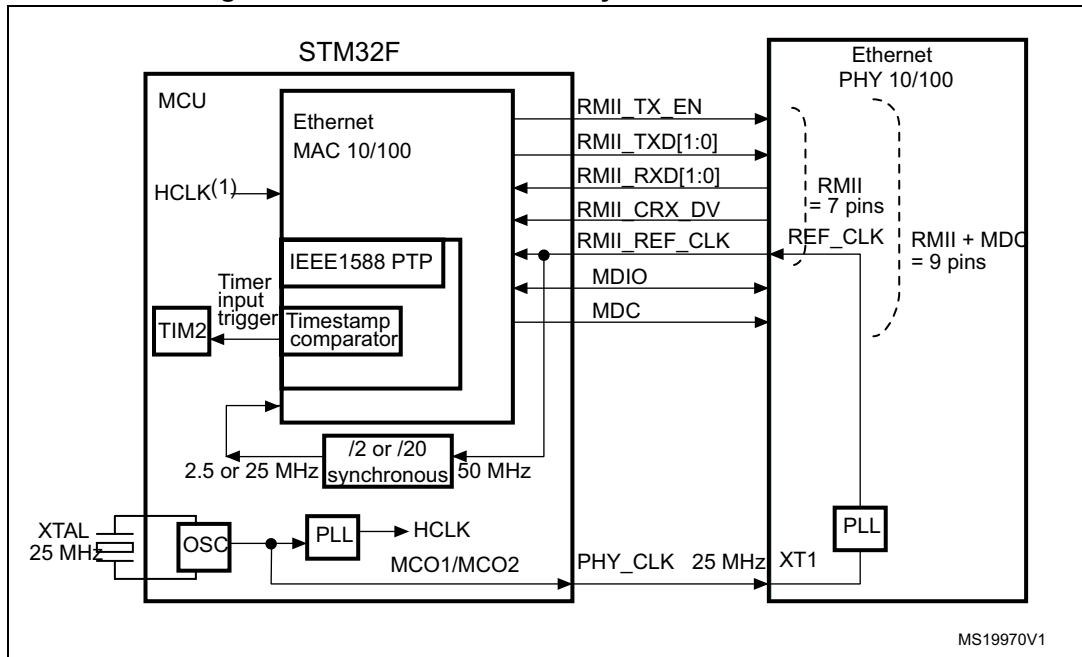
Figure 99. RMI1 with a 25 MHz crystal and PHY with PLL
