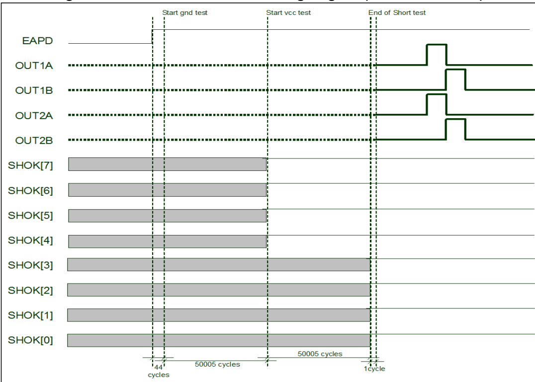
Figure 23. Short-circuit detection timing diagram (no short detected)
