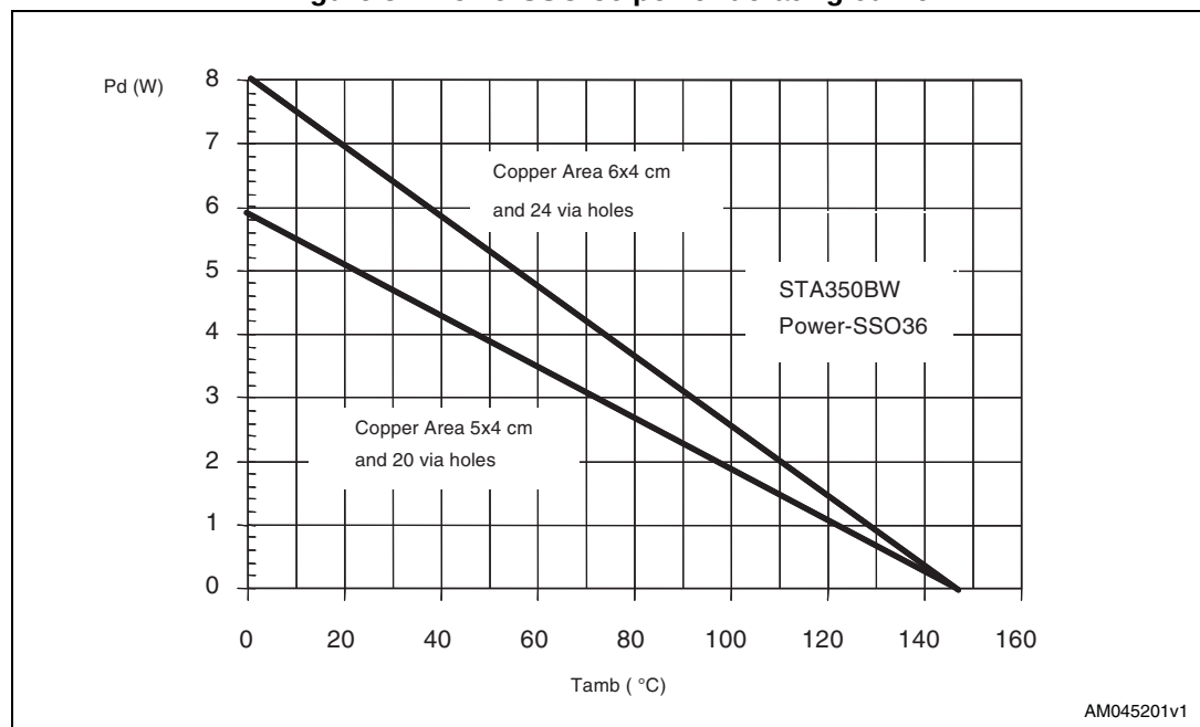
Figure 37. PowerSSO-36 power derating curve
