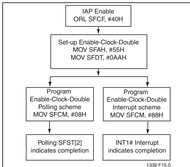
FIGURE 4-8: Enable-Clock-Double
