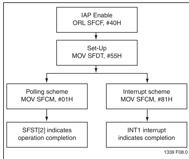
FIGURE 4-1: Chip-Erase
