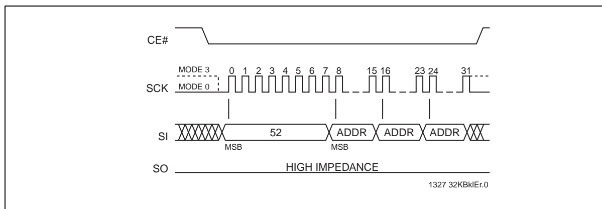
Figure 13: 32-KByte Block-Erase Sequence
