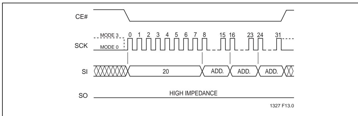
Figure 12: Sector-Erase Sequence
