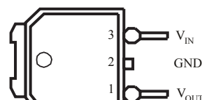
TO-252 (R)
