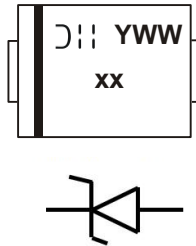
Cathode Band for Unidirectional Device
