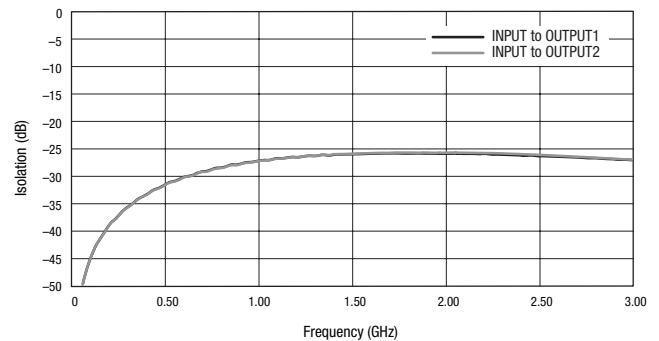
Figure 4. Typical Isolation
