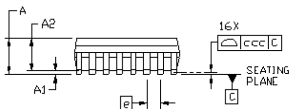
Figure 10.1. 16-Pin QSOP Package
