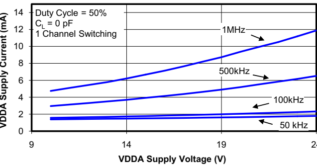
Figure 24. Supply Current vs. Supply Voltage
