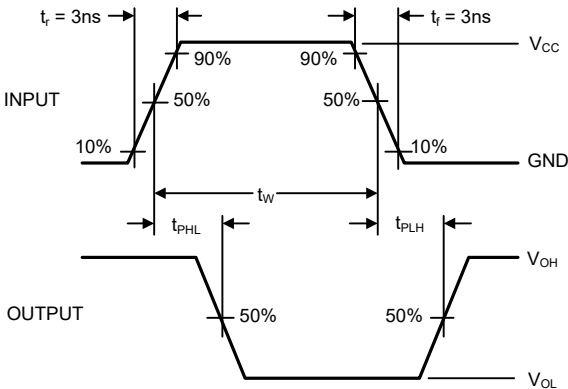
Figure 2. AC Waveforms
