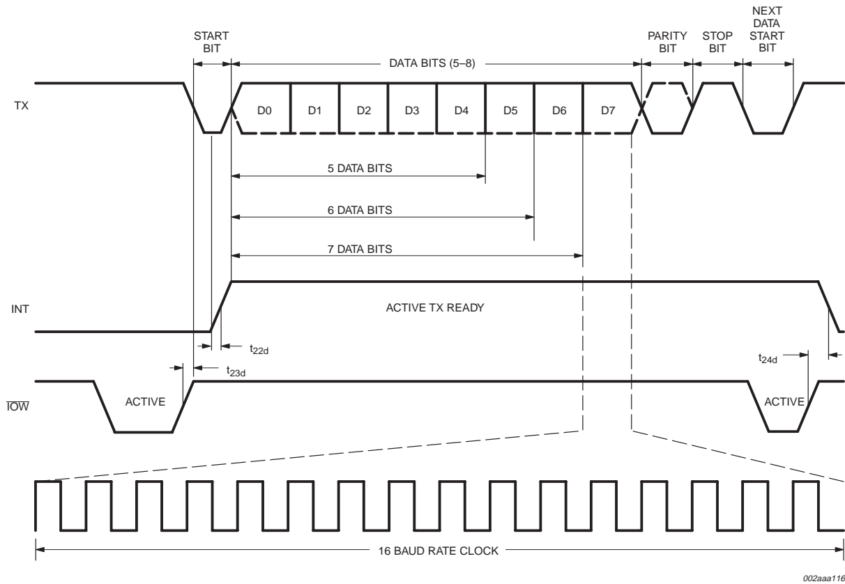
Fig 20. Transmit timing.
