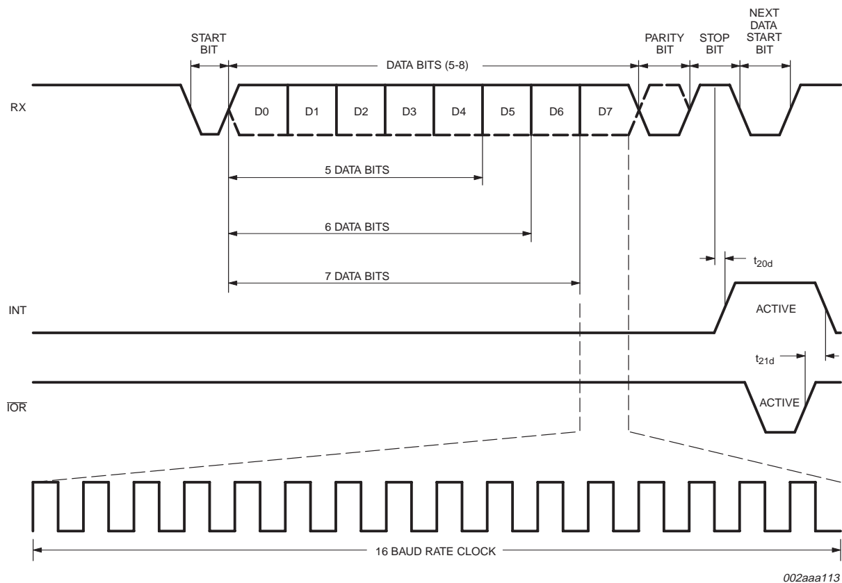
Fig 17. Receive timing.
