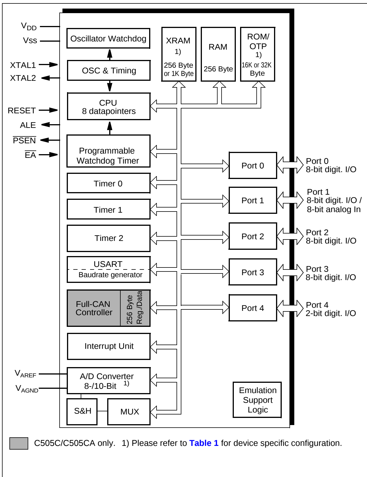
Figure 4 Block Diagram of the C505/C505C/C505A/C505CA
