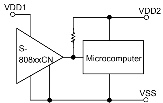
Figure 28 Reset Circuit Example (S-808xxCN)
