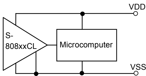
Figure 27 Reset Circuit Example(S-808xxCL)
