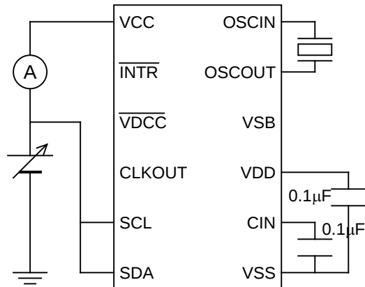
Test circuit
