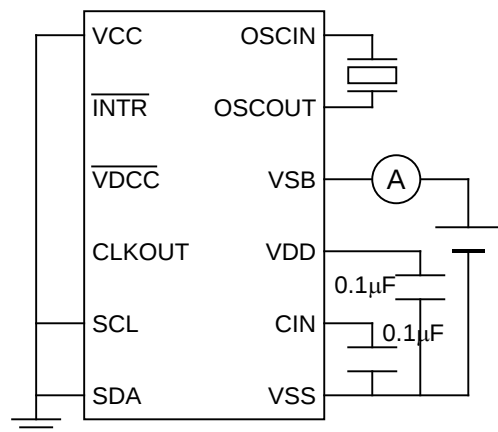
Test circuit
