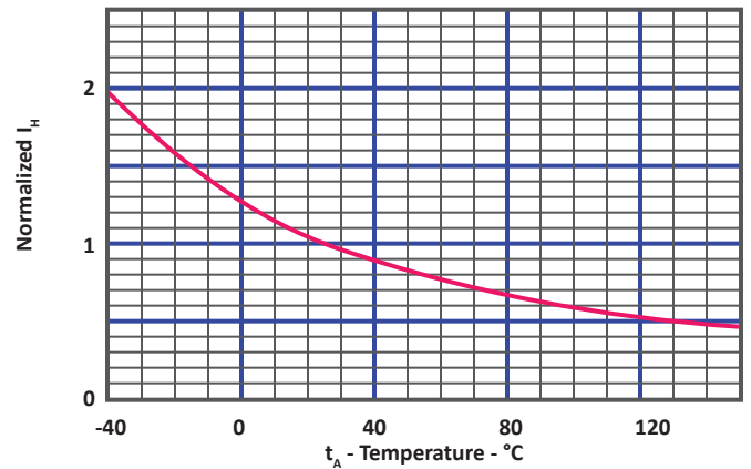
FIGURE 7 TYPICAL NORMALIZED HOLDING CURRENT VS JUNCTION TEMPERATURE
