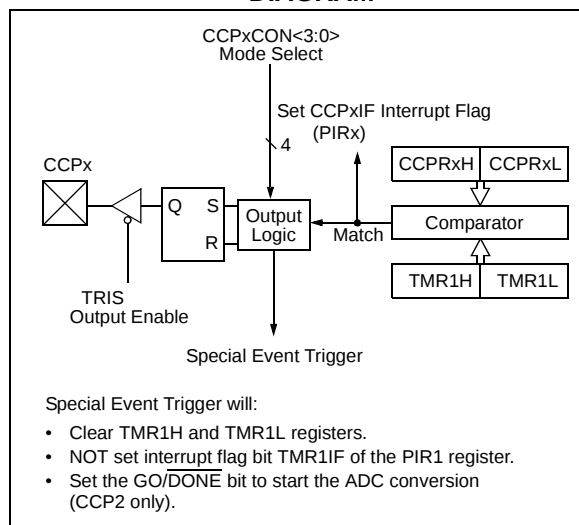
FIGURE 15-2: COMPARE MODE OPERATION BLOCK DIAGRAM
