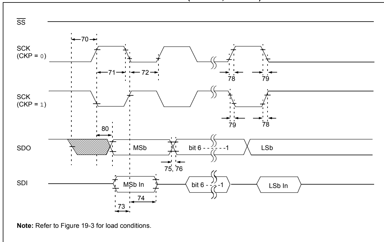
FIGURE 19-15: SPI MASTER MODE TIMING (CKE = 1, SMP = 1)
