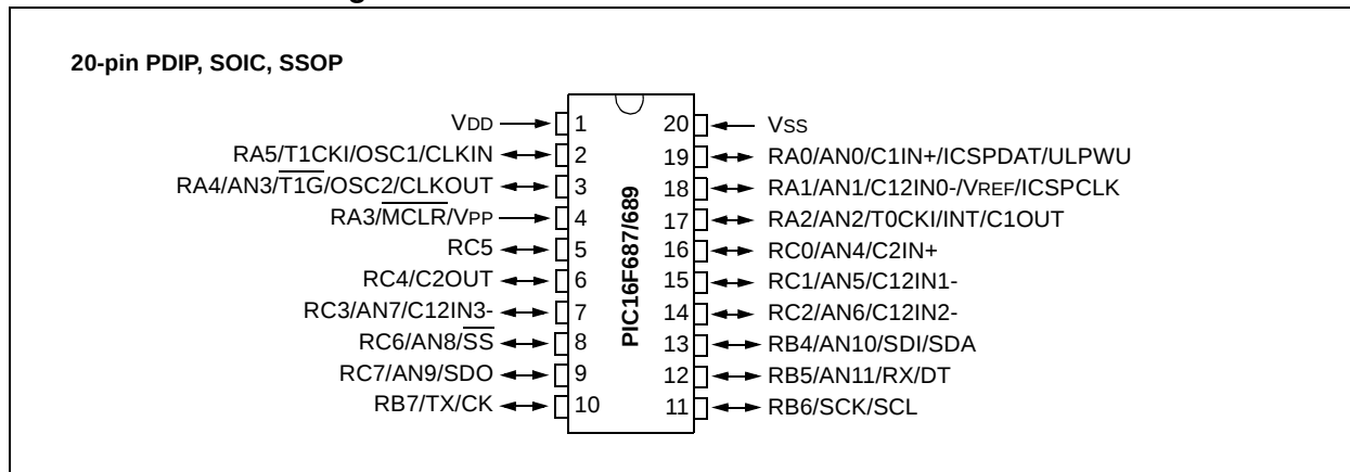
PIC16F687/689 Pin Diagram
