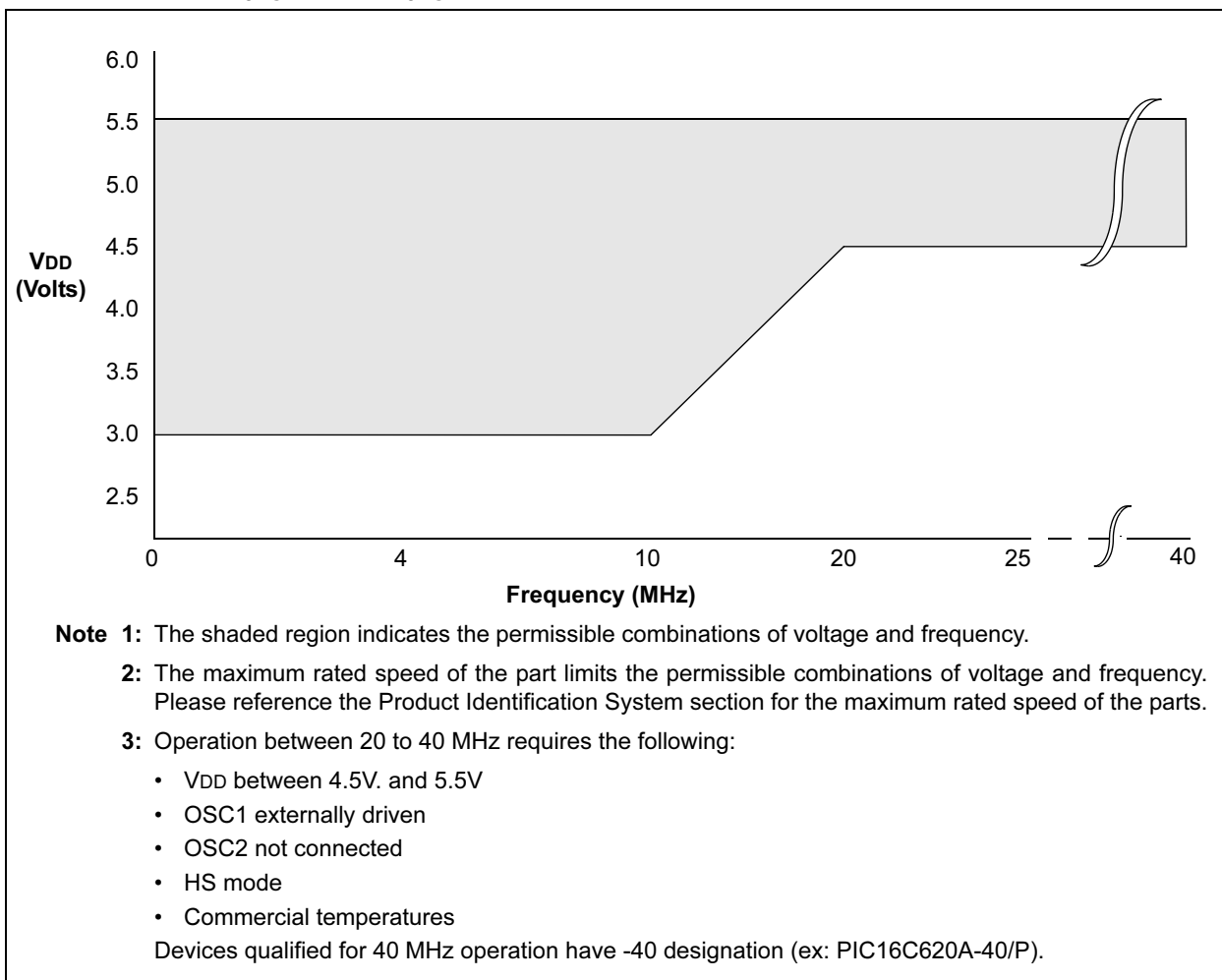
FIGURE 12-10: PIC16C620A/C621A/C622A/CR620A - 40 VOLTAGE-FREQUENCY GRAPH, 0^{\circ}\text{C} \leq T_A \leq +70^{\circ}\text{C}
