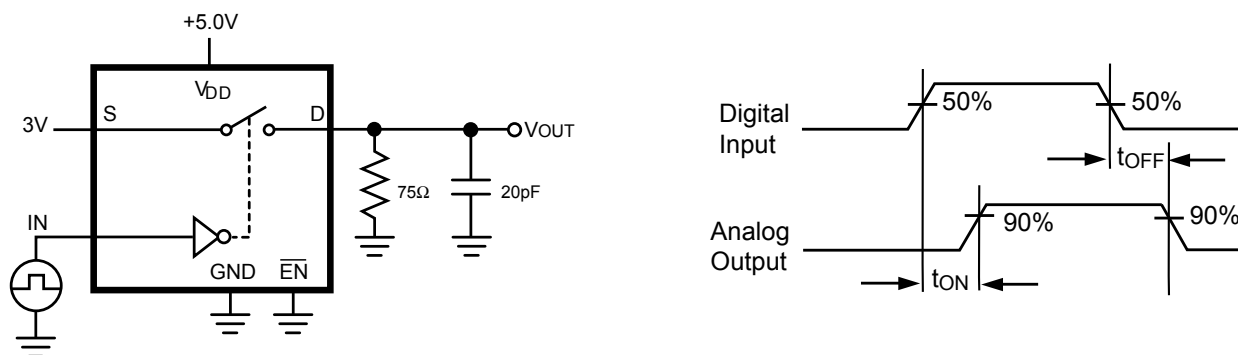
Figure 4. Switching Time
