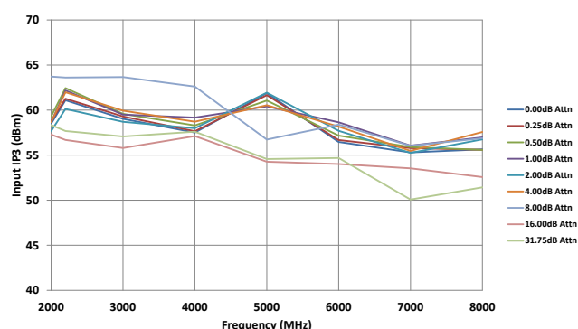
Figure 29. IIP3 vs. Attenuation Setting
