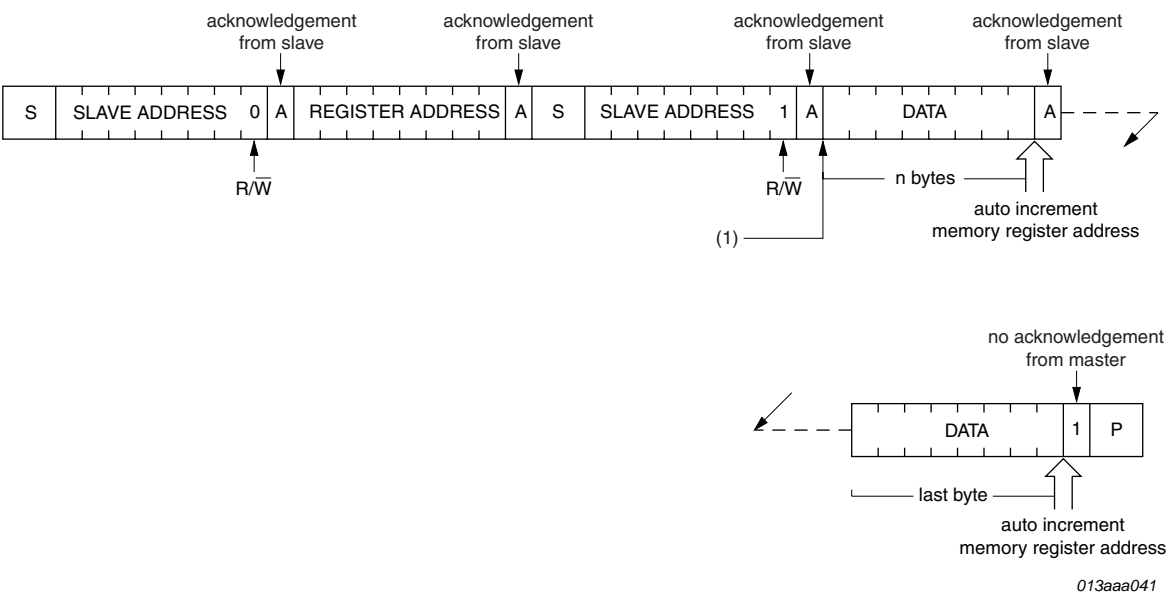
Fig 18. Master reads after setting register address (write register address; READ data)
