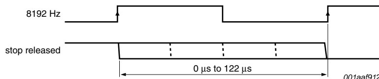
Fig 10. STOP bit release timing
