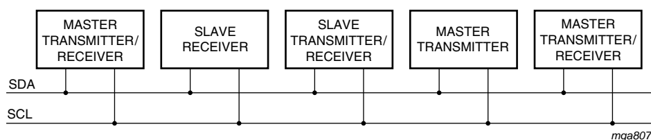
Fig 14. System configuration
