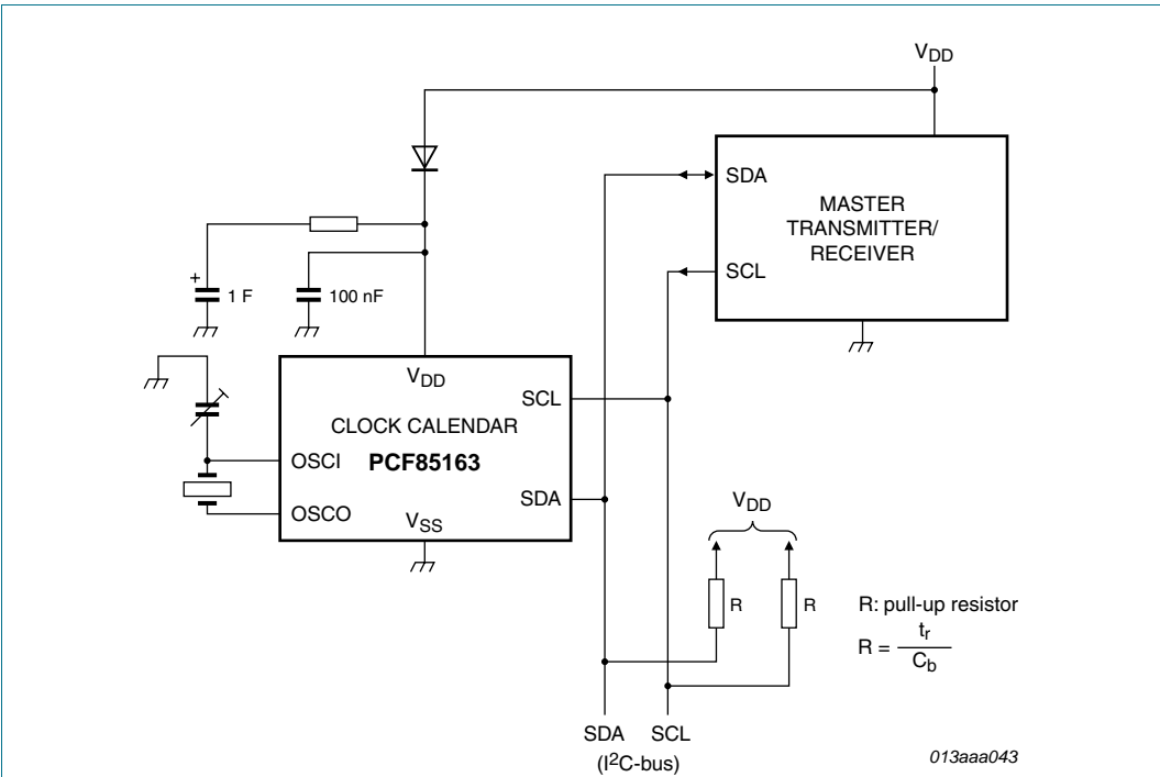
Fig 25. Application diagram
