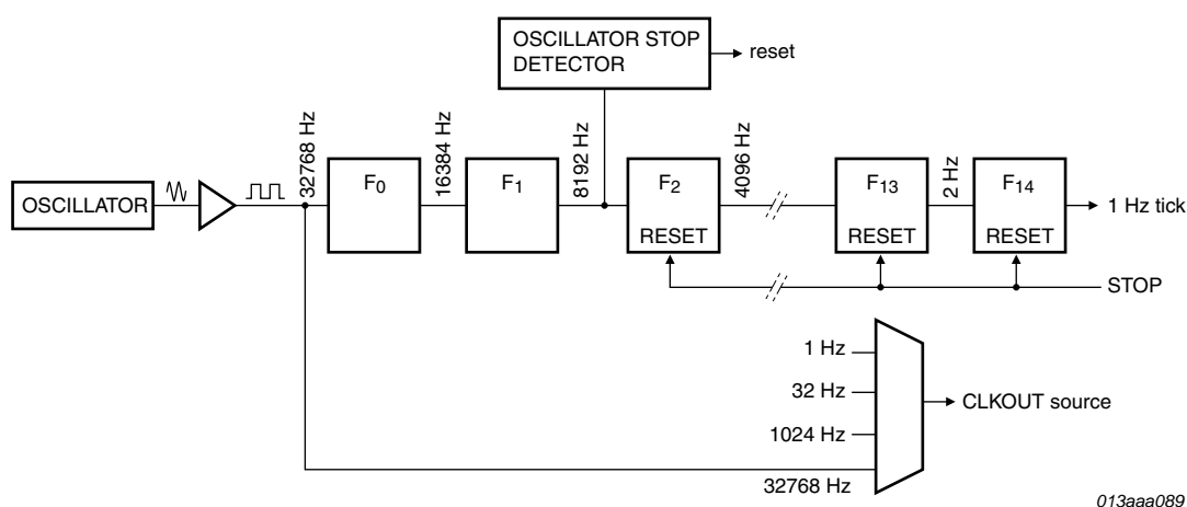
Fig 9. STOP bit functional diagram
