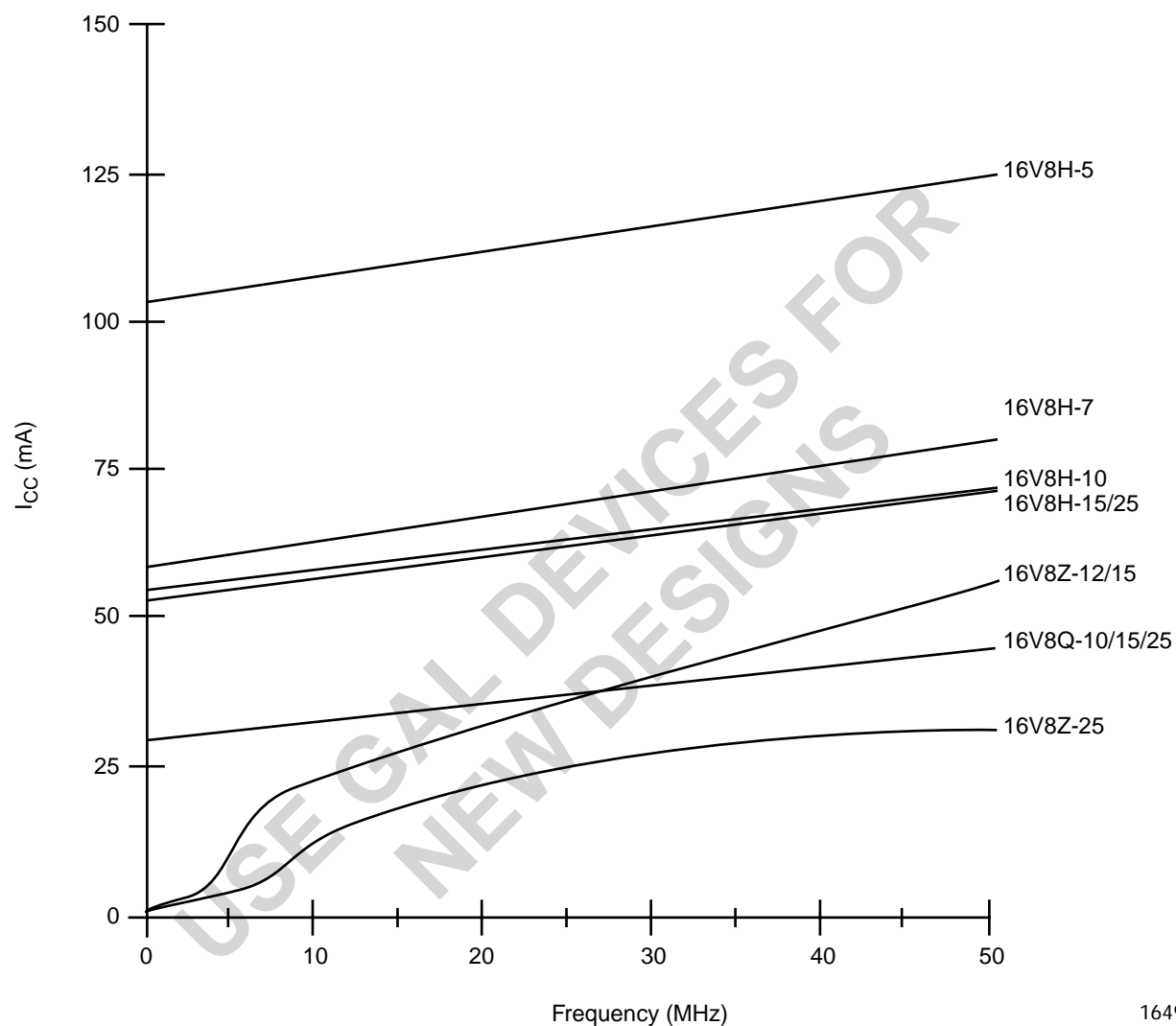
I_{CC} vs. Frequency
