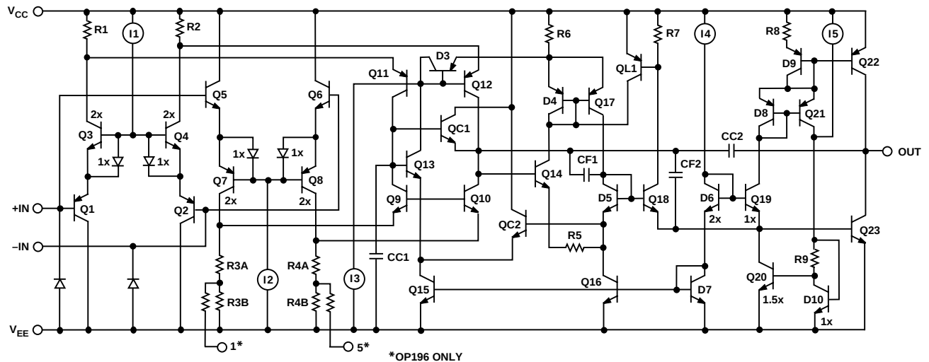
TPC 36. Simplified Schematic
