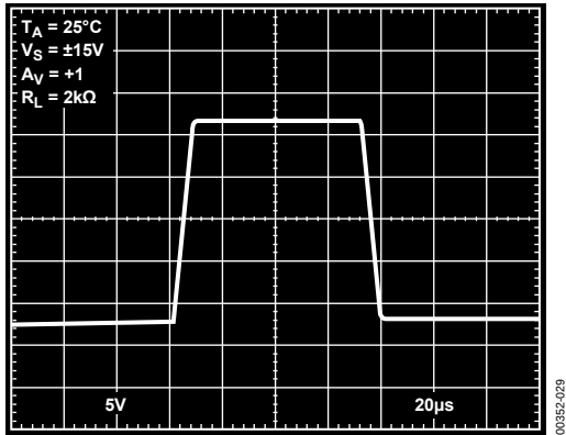
Figure 28. Large-Signal Transient Response
