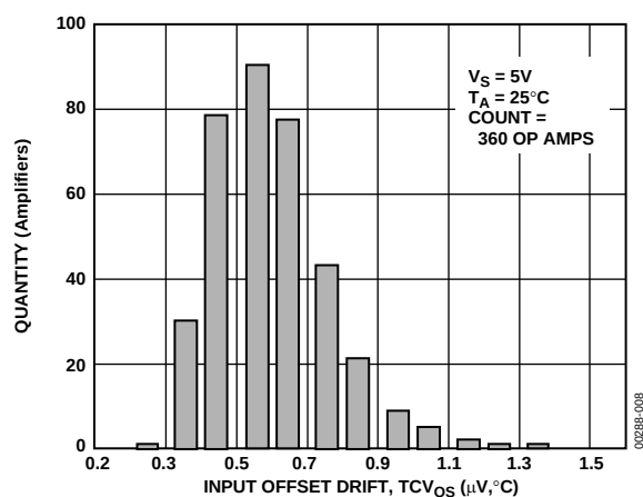
Figure 5. OP462 Input Offset Voltage Drift ( \text{TCV}_{OS} )
