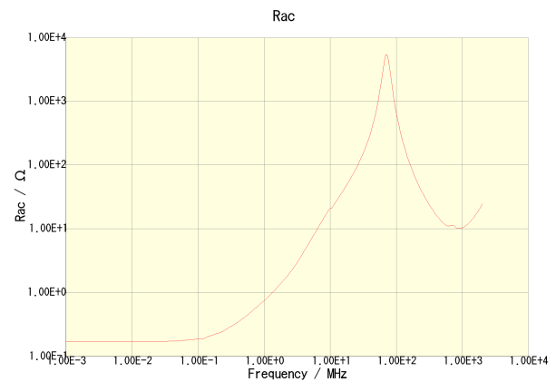
NLCV32T-3R3M-PF
