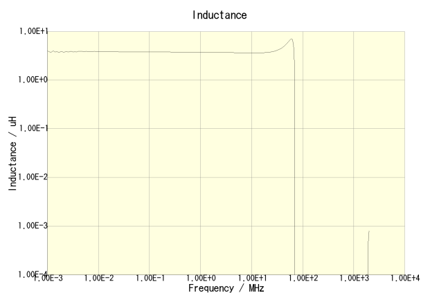
NLCV32T-3R3M-PF
