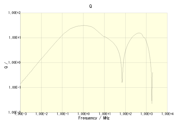
NLCV32T-3R3M-PF
