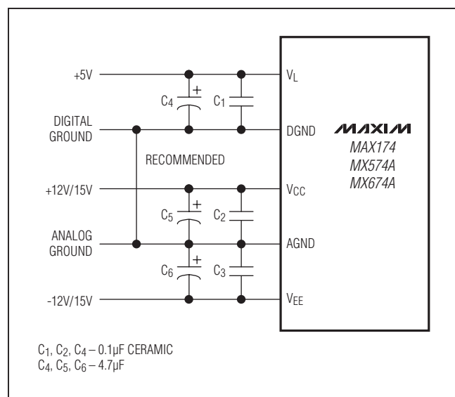
Figure 9. Power-Supply Bypassing
