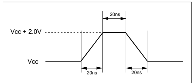
Figure 37. Maximum Positive Overshoot Waveform
