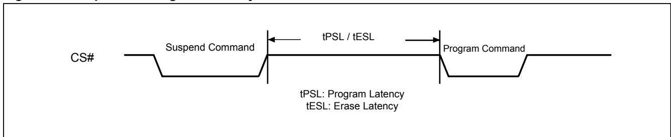
Figure 32. Suspend to Program Latency
