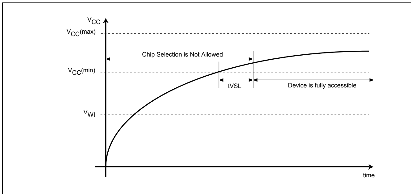
Figure 44. Power-up Timing
