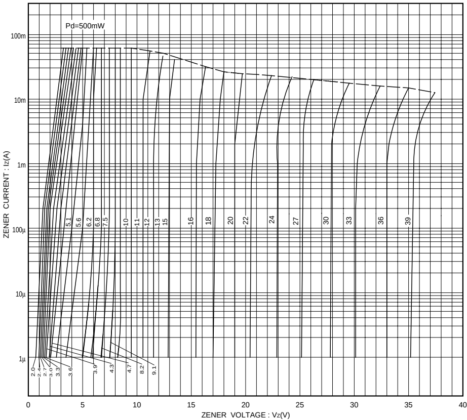
Fig. 1 Zener characteristics
