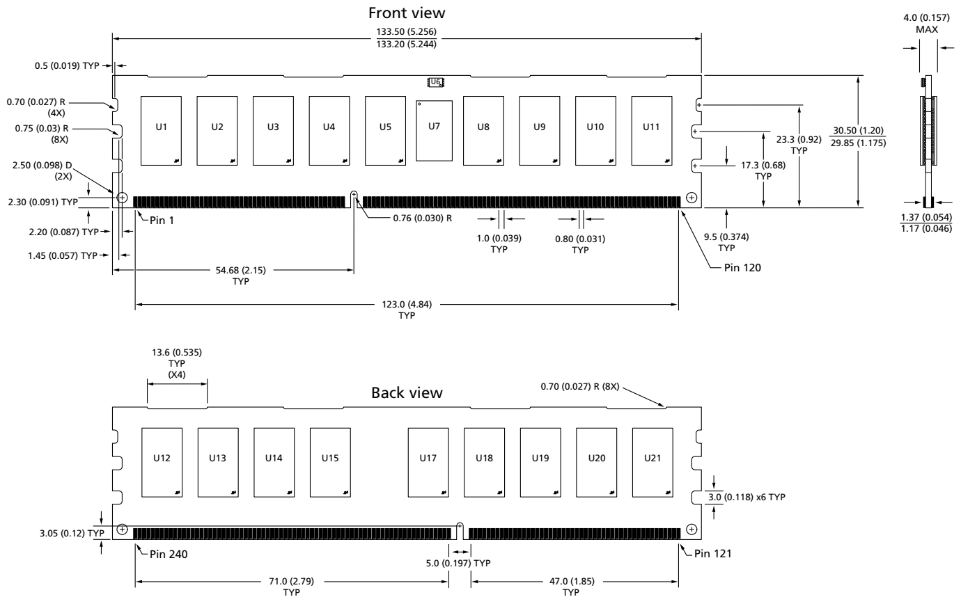
Figure 5: 240-Pin DDR3 RDIMM R/C B (PCB 0693)
