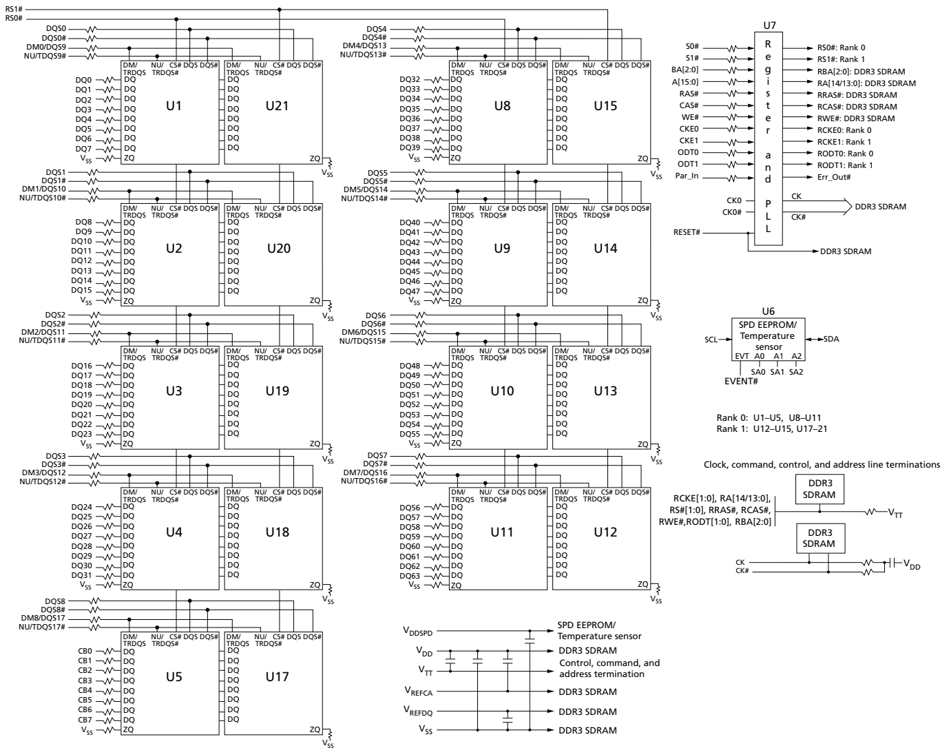
Figure 3: Functional Block Diagram R/C B (PCB 0693)
