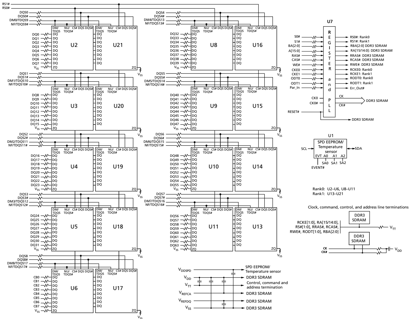
Figure 4: Functional Block Diagram R/C B1(PCB 1164, 1382 and 1560)
