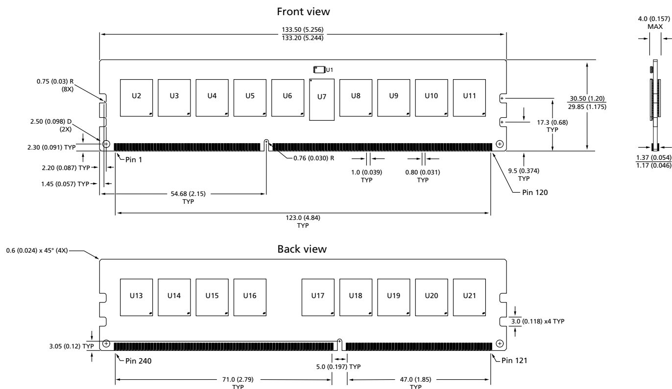
Figure 7: 240-Pin DDR3 RDIMM R/C B1 (PCB 1560)
