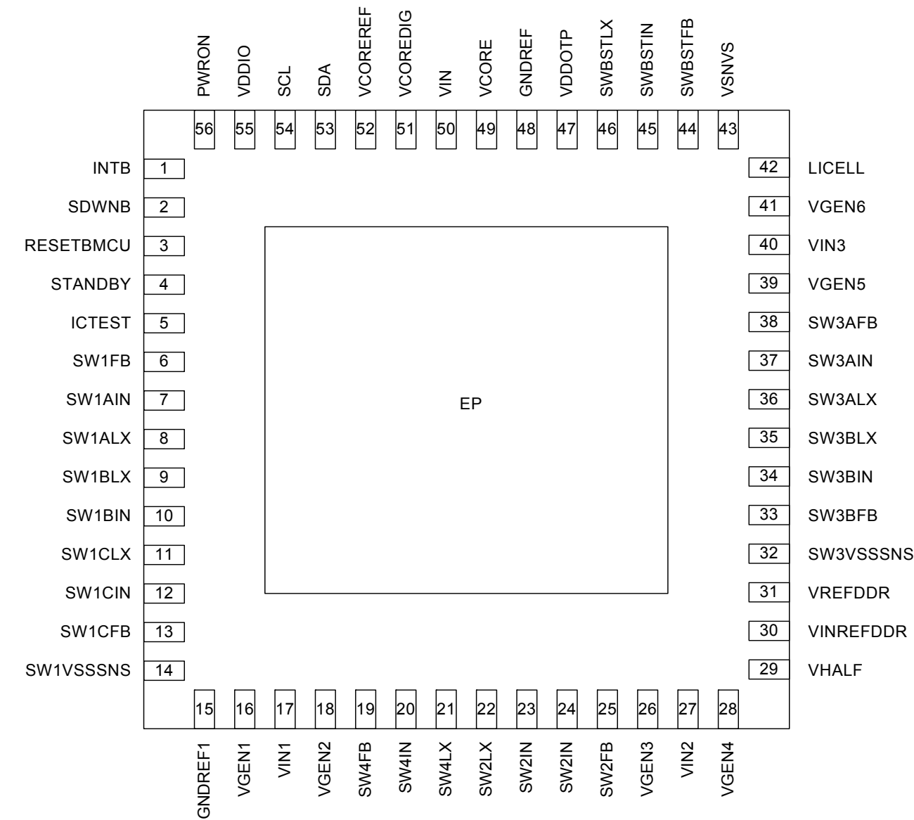
Figure 3. Pinout diagram
