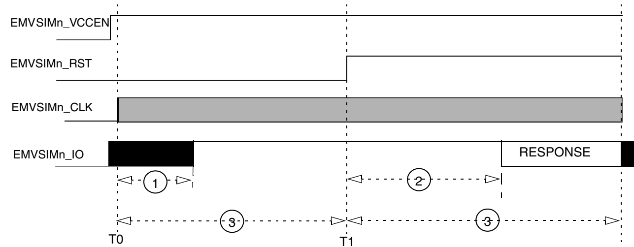
Figure 32. Active-Low-Reset Smart Card Reset Sequence
