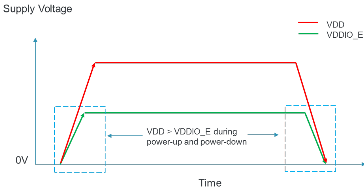
Figure 3. VDD > VDDIO_E
