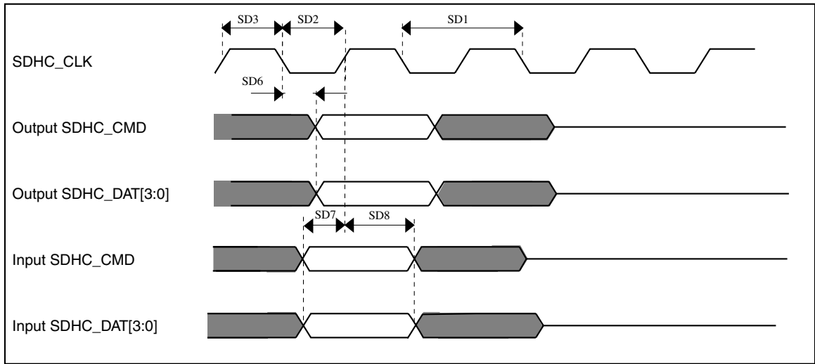
Figure 26. SDHC timing
