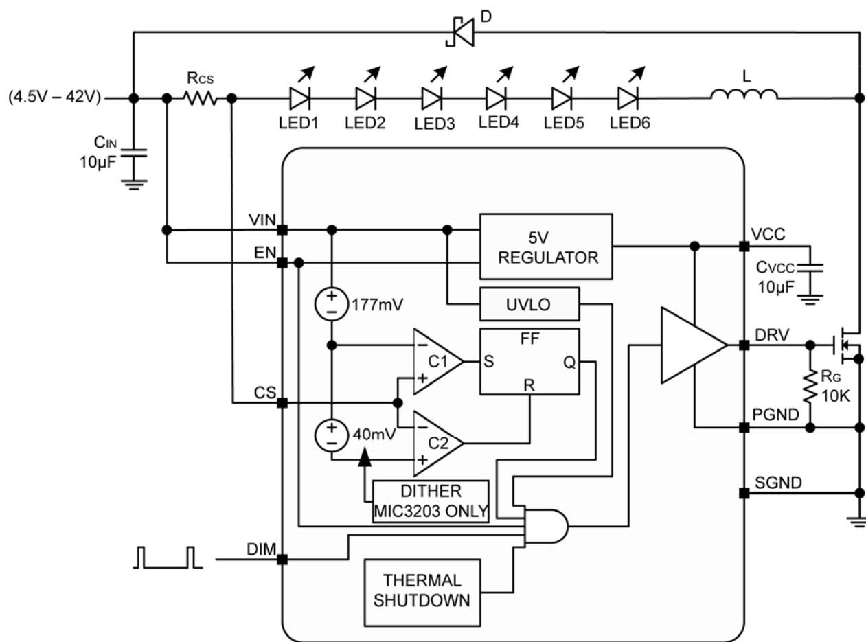
Figure 1. MIC3203/MIC3203-1 Block Diagram
