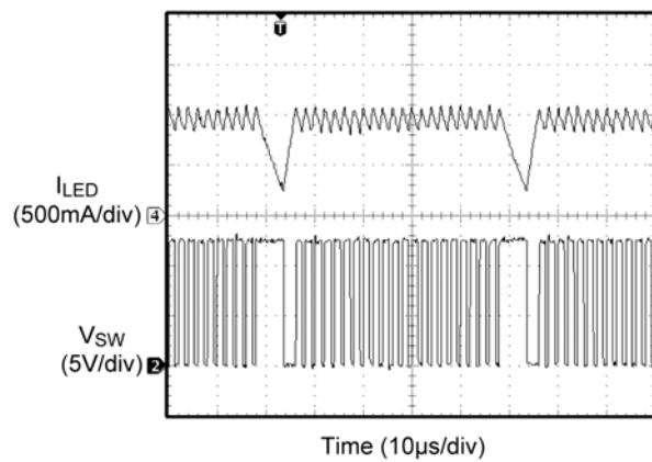
PWM Dimming @ 20kHz (10% Duty Cycle)
