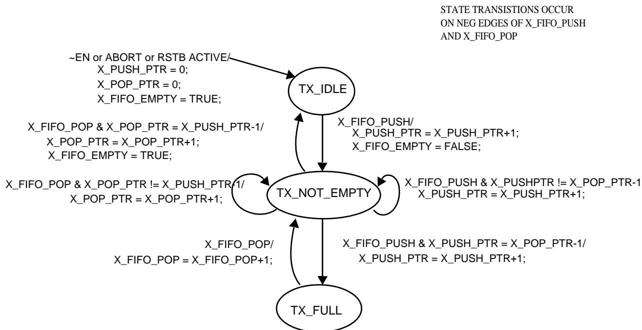
Figure 22. State Diagram of Transmit FIFO
