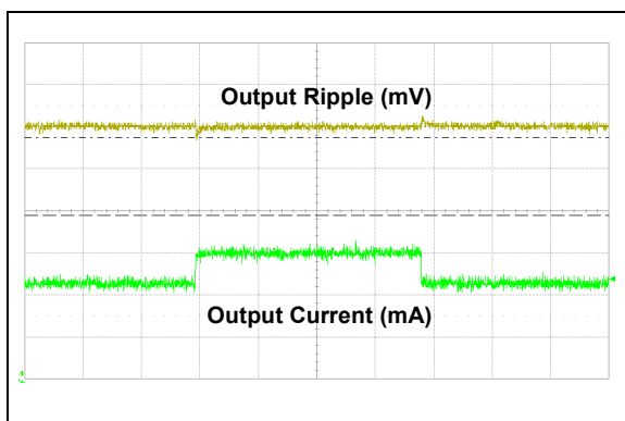
FIGURE 2-15: Load Transient Response ( I_{LOAD} = 50\text{ mA} , Output: 100 mV/Div, Time: 100 μs/Div).
