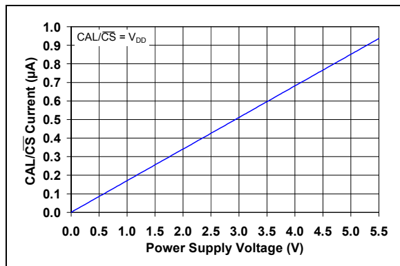
FIGURE 2-44: CAL/CS Current vs. Power Supply Voltage.
