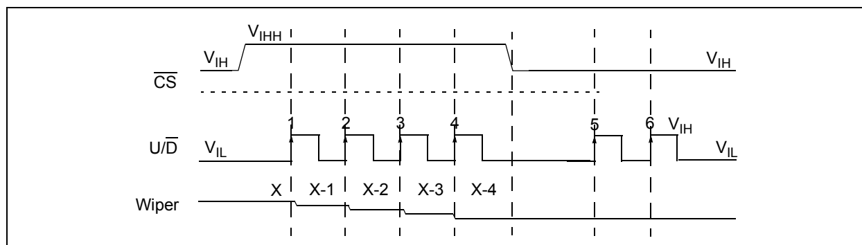
FIGURE 5-7: High-Voltage Decrement 1 (For MCP402X Compatibility).
