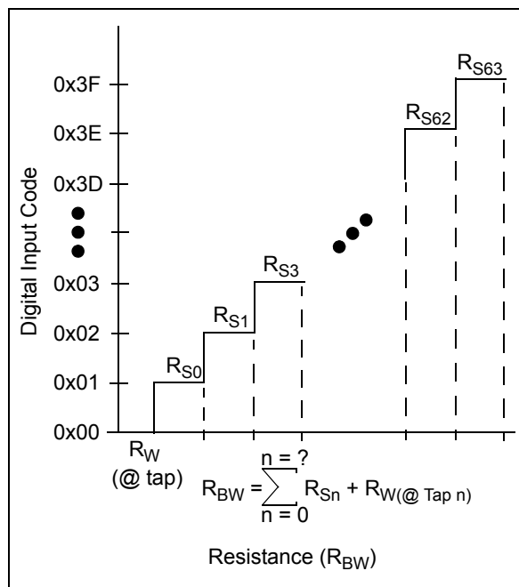
FIGURE 6-7: Resistance R_{BW} .
