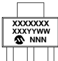
3-Lead SOT-223
