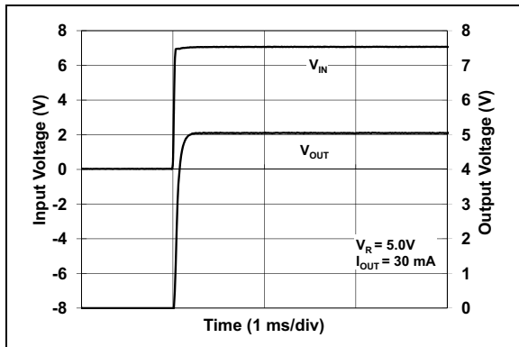
FIGURE 2-37: Start-up Response.
