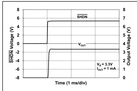
FIGURE 2-40: SHDN Response.
