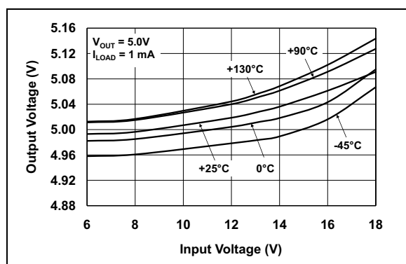
FIGURE 2-9: Output Voltage vs. Input Voltage.
