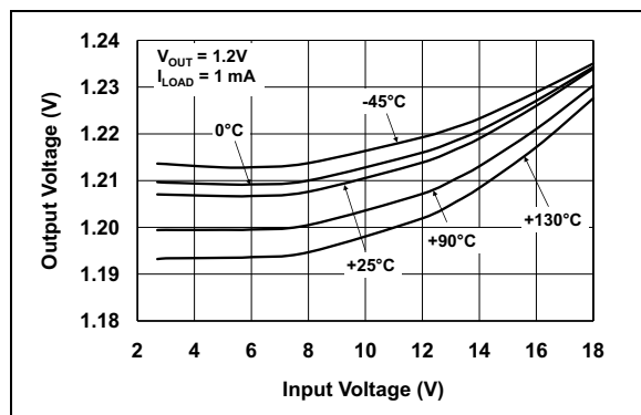
FIGURE 2-7: Output Voltage vs. Input Voltage.
