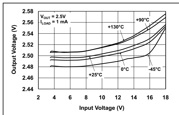
FIGURE 2-8: Output Voltage vs. Input Voltage.
