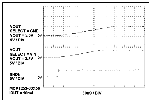
FIGURE 2-18: Start-Up (MCP1253-33X50).
