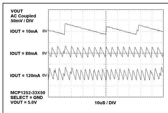
FIGURE 2-16: Output Voltage Ripple vs. Time.
