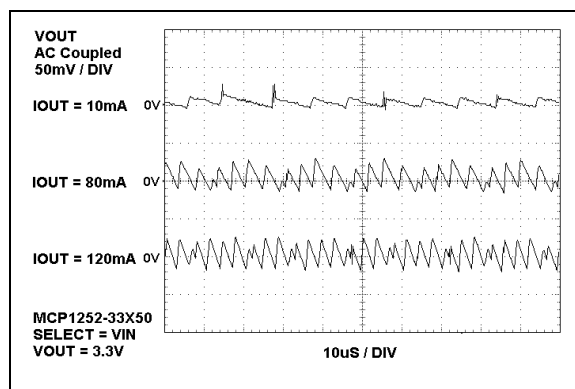
FIGURE 2-17: Output Voltage Ripple vs. Time.
