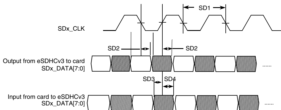
Figure 41. eMMC4.4/4.41 Timing
