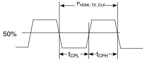
Figure 54. TMD5 Clock Signal Definitions
