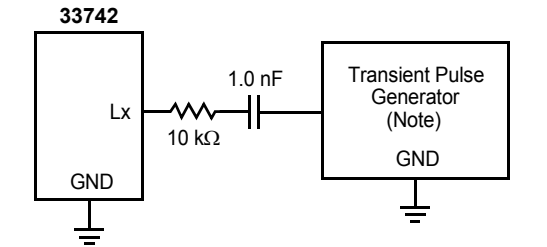
Note Waveform per ISO 7637-1. Test Pulses 1, 2, 3a, and 3b. Figure 5. Transient Test Setup for L0:L3 Inputs
