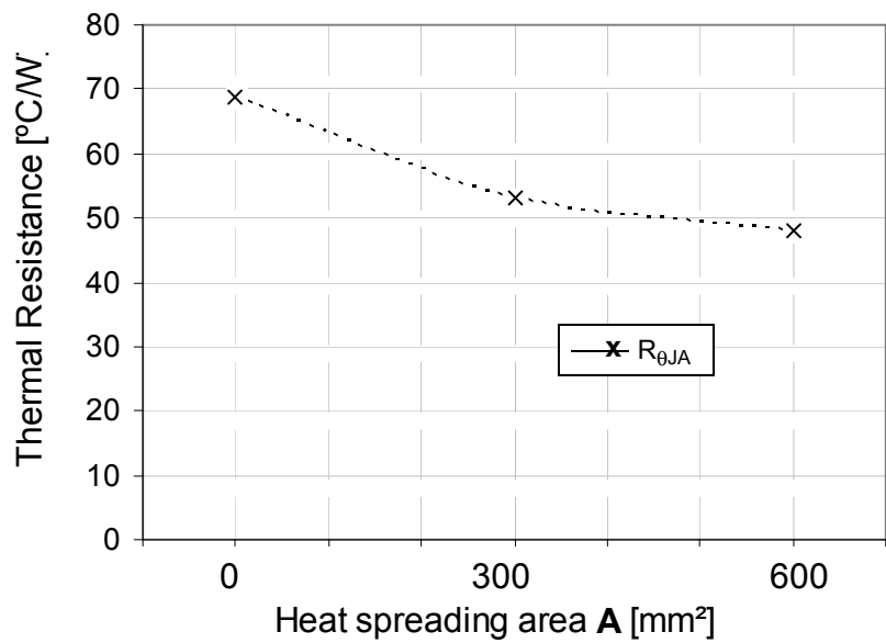
Figure 27. Device on thermal test board R θJA
